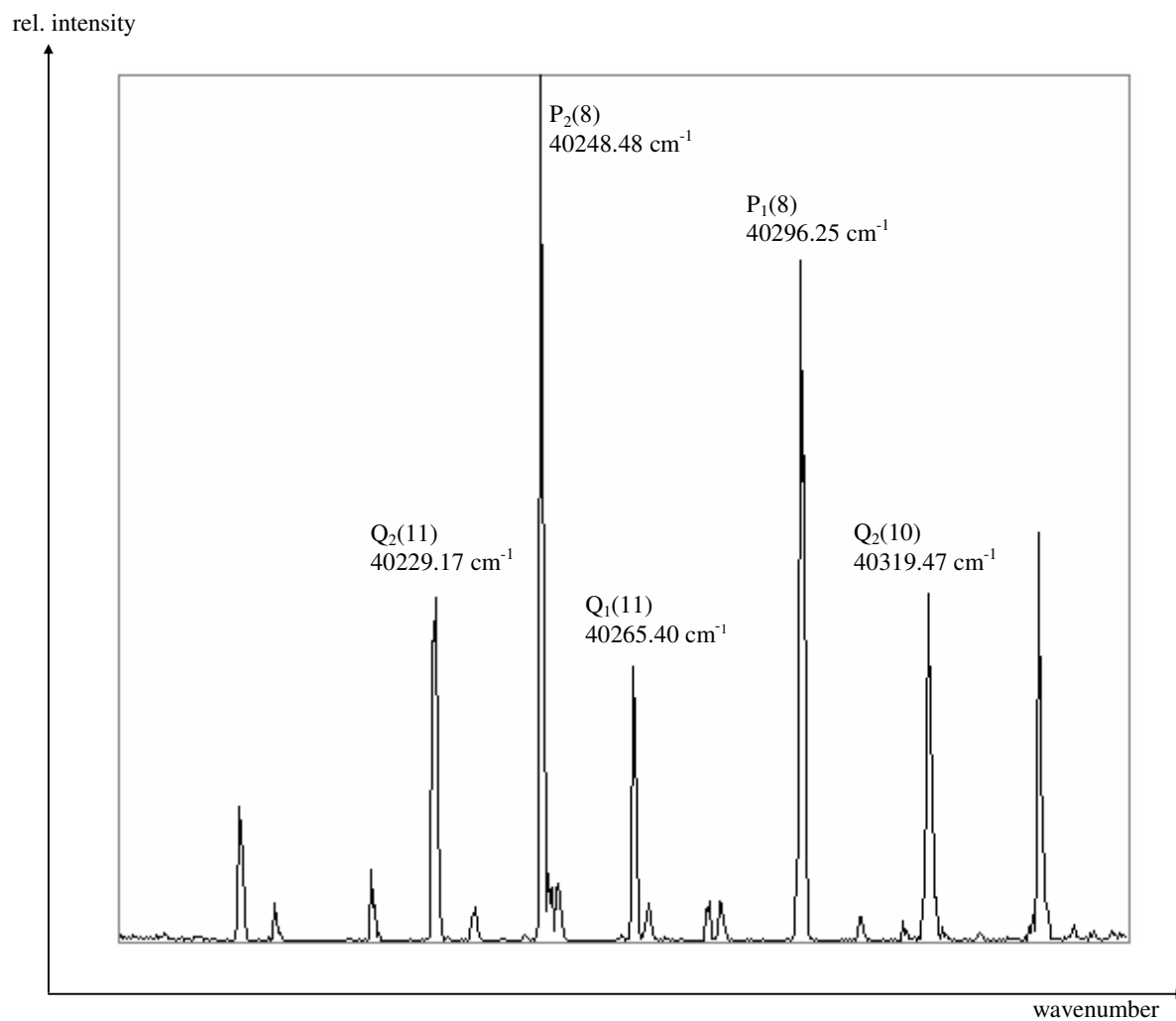
Fig. 4: Excitation spectra of the OH-radical at 248 nm captured by IICCD-camera and 18 MHz pixel-clock
