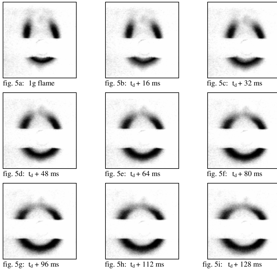
Fig. 5a-5i: Image sequence with 1g \rightarrow \mu g transition at 250 Hz (each 4th image is shown)
