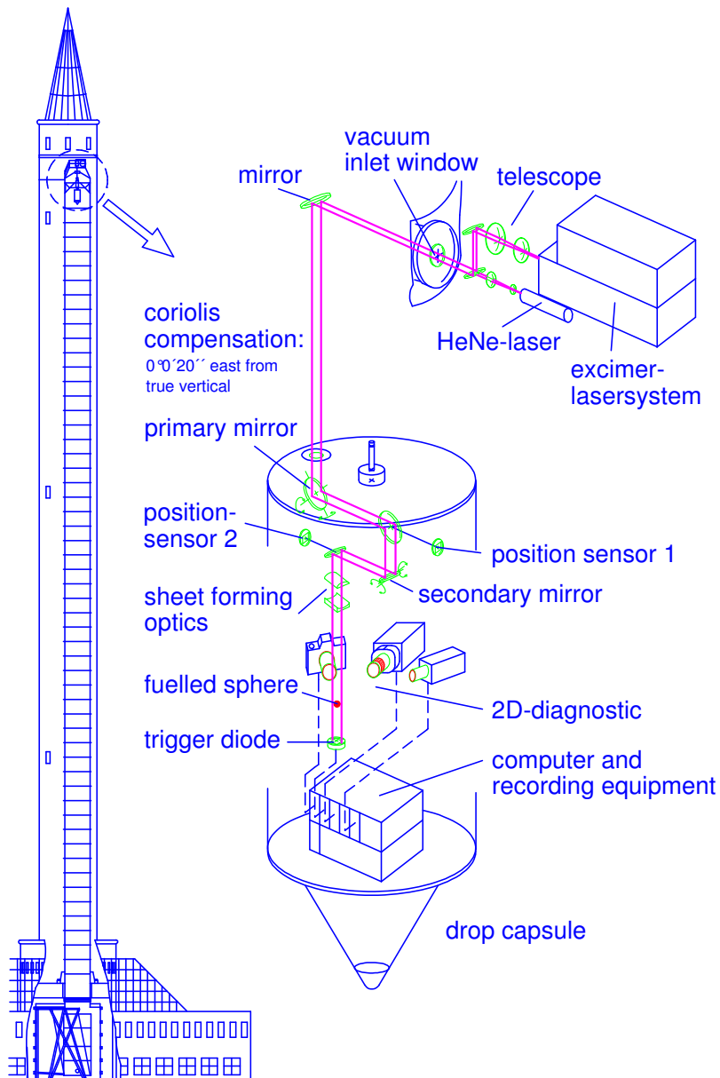
Fig. 1: Drop tower with drop capsule and beam guide of UV-lasersystem
